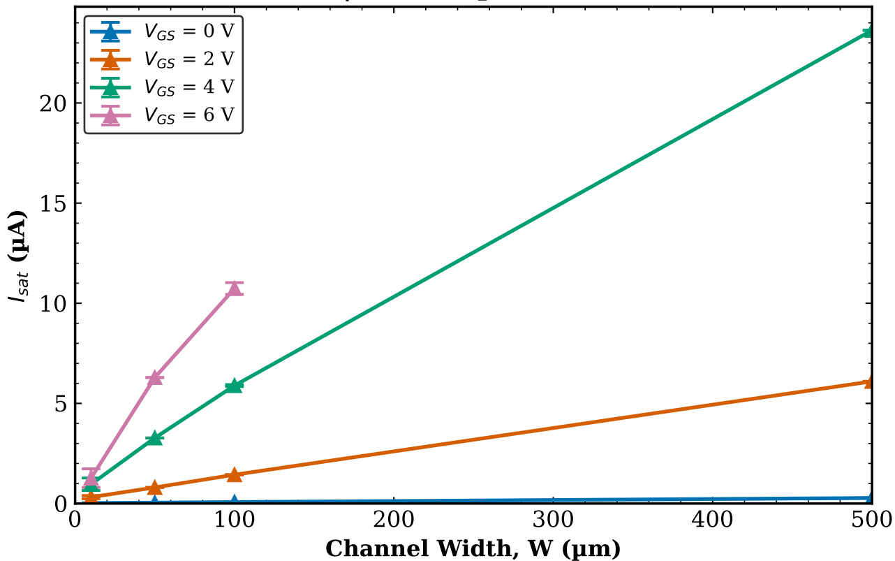
TFT2 Combined (Tr. 1 & 2) I_{sat} vs W | L = 80\text{ }\mu\text{m} (mean \pm std)
